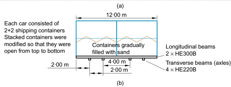
Fig. 7. (a) Test site and containers before loading; (b) container layout used to simulate train car loading pattern
